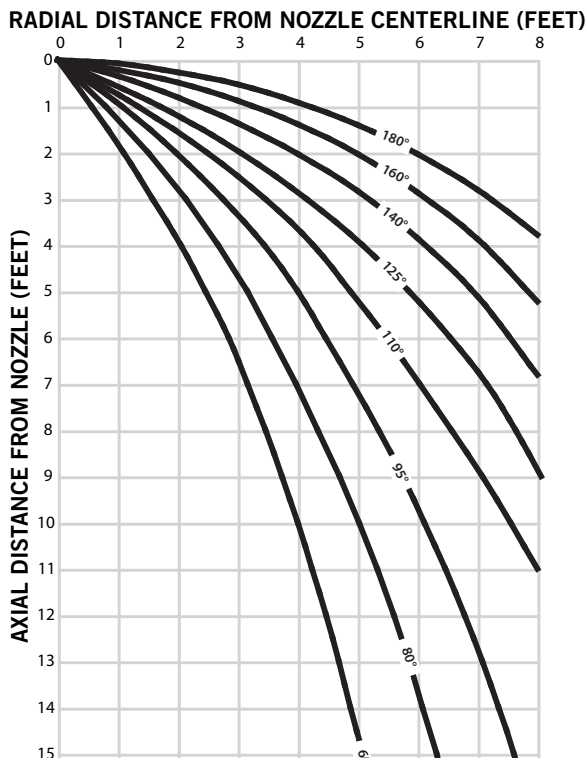
Figure 2 - Design Spray Profiles (All K Factors)
