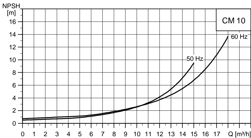
Фиг. 6 NPSH curves for CM 10
