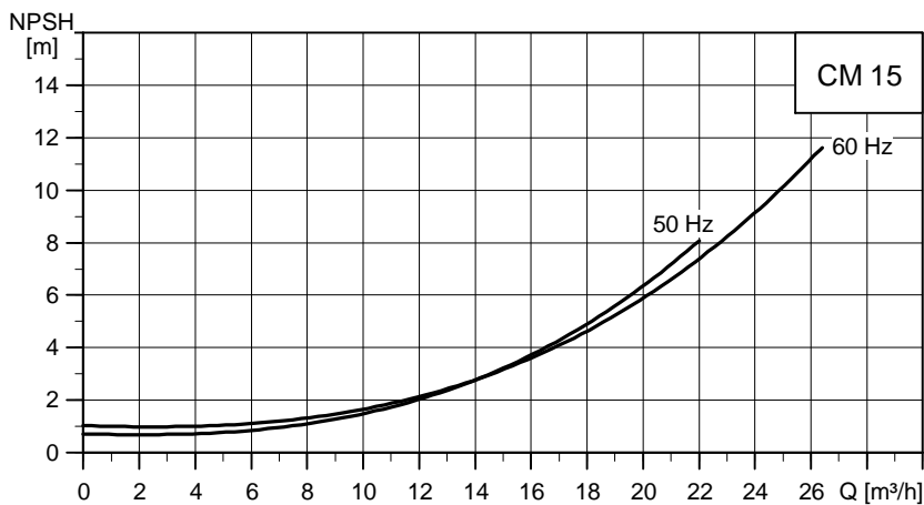
Фиг. 7 NPSH curves for CM 15
