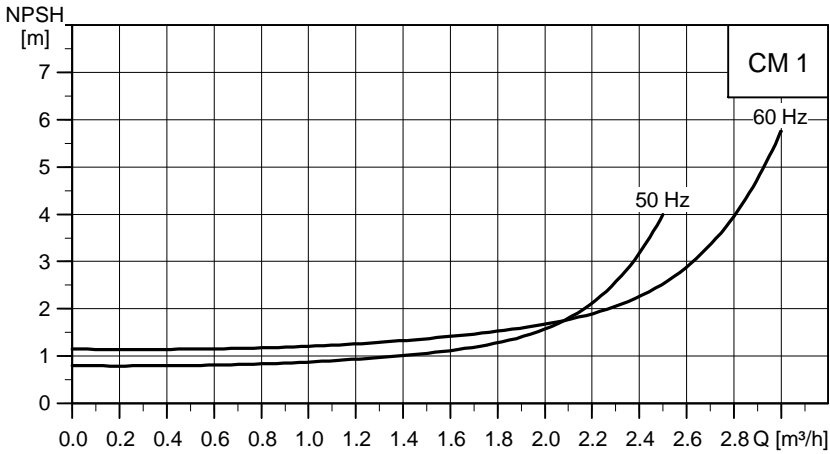
Фиг. 4 NPSH curve for CM 1
