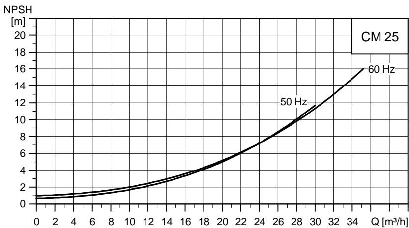
Фиг. 8 NPSH curves for CM 25
